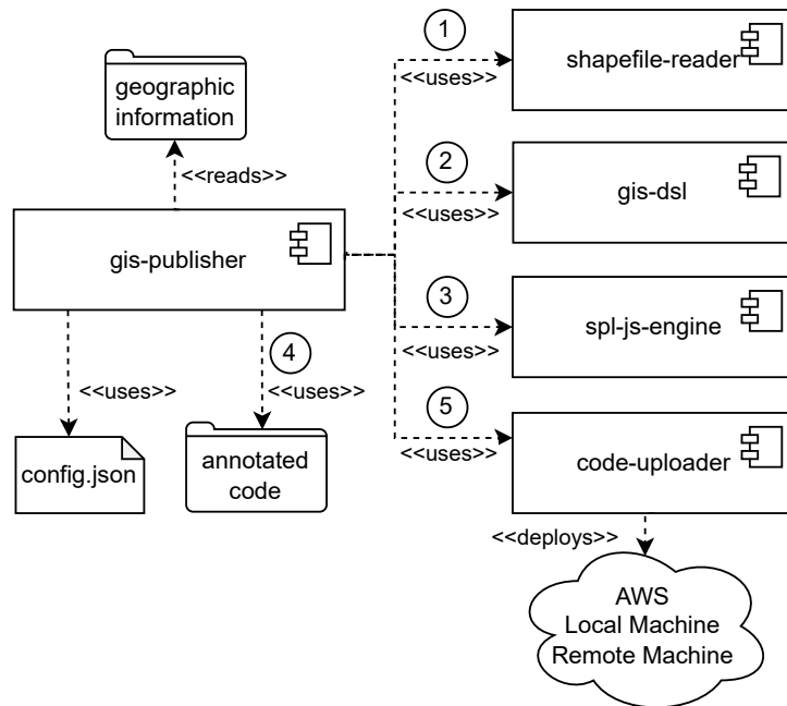
Figure 1: Component diagram of the tool architecture
